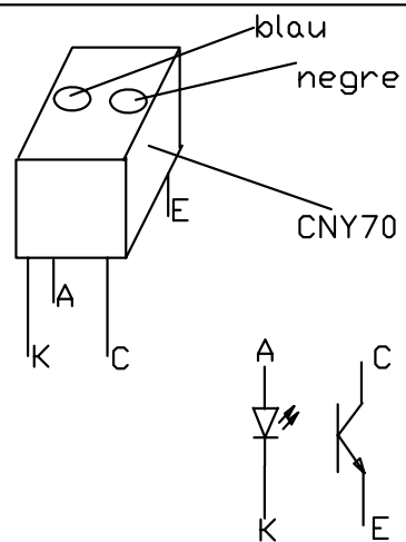
Sensor CNY70
