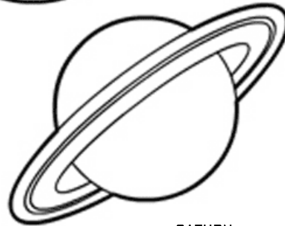
SATURN
